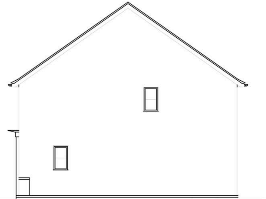
SIDE ELEVATION Chester
